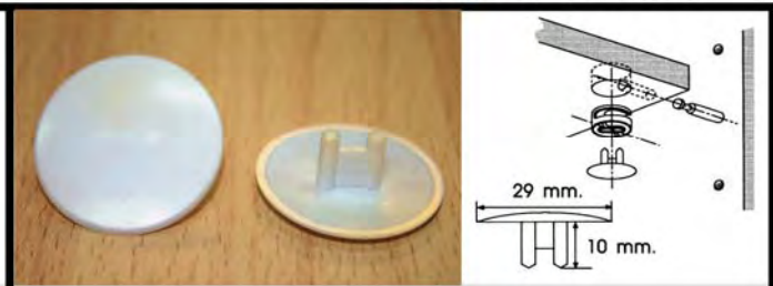
PLASTIC COVER CAP / ฝาปิด EXCENTER
